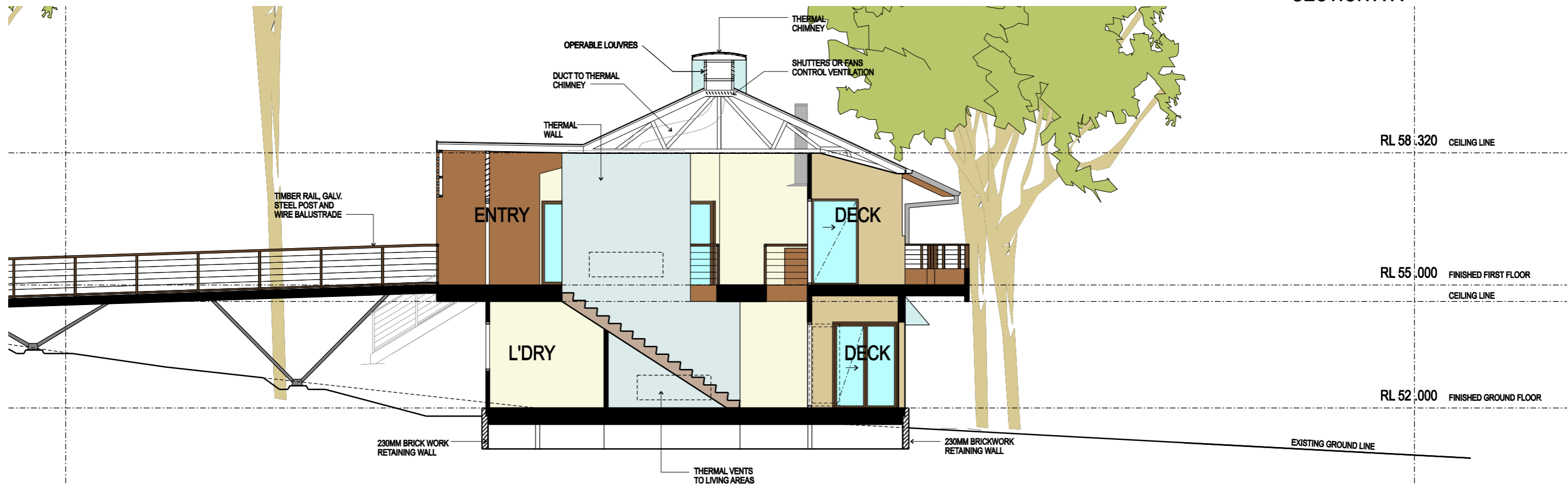
SECTION B-B
