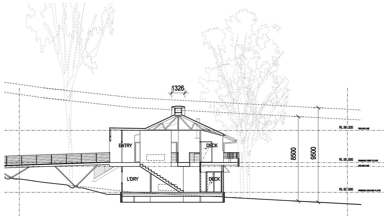
SECTION B-B
