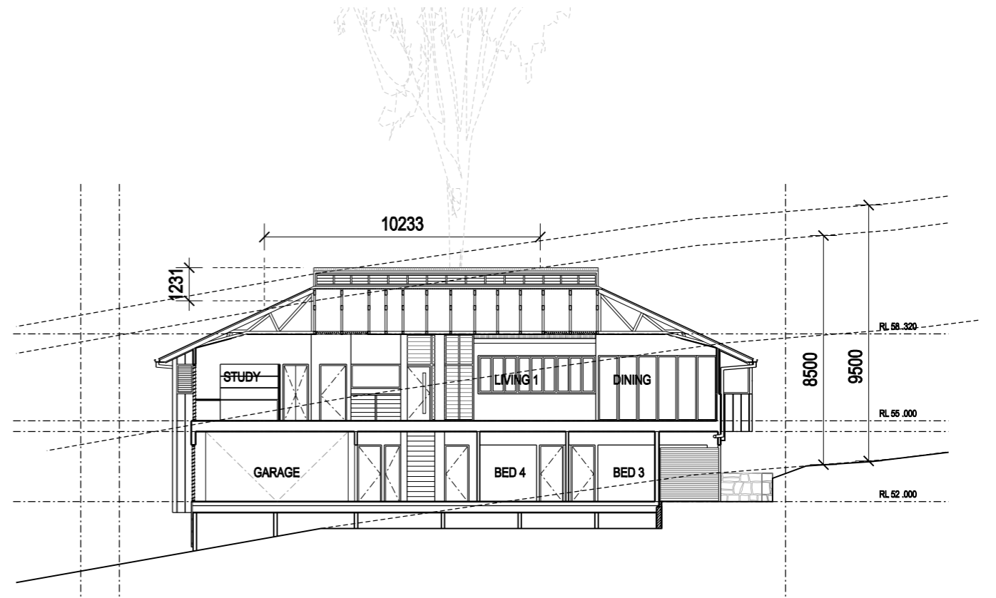
SECTION C-C
