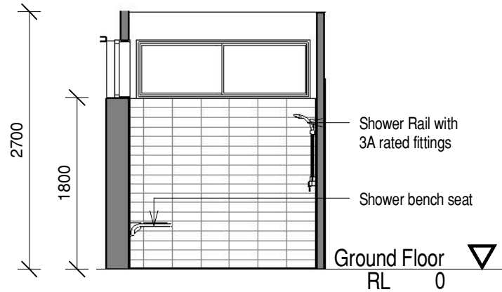
C Bathroom 1 - Elevation C 1 : 50
