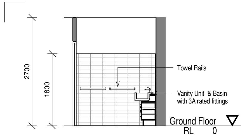
A Bathroom 1 - Elevation A 1 : 50
