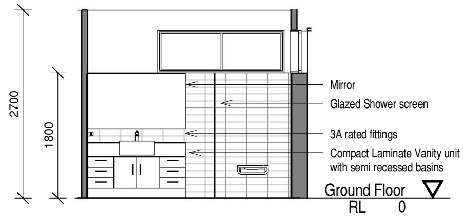
B Bathroom 1 - Elevation B 1 : 50
