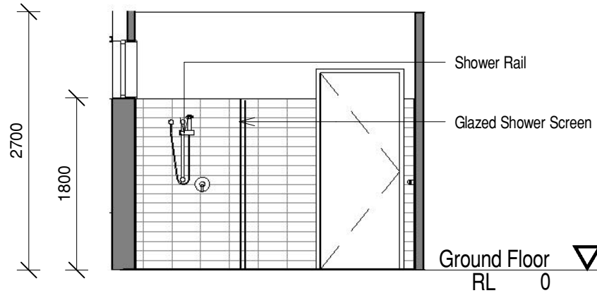
D Bathroom 1 - Elevation D 1 : 50
