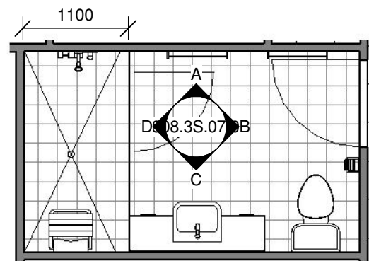
1 Bathroom 2 Floor Plan 1 : 50
