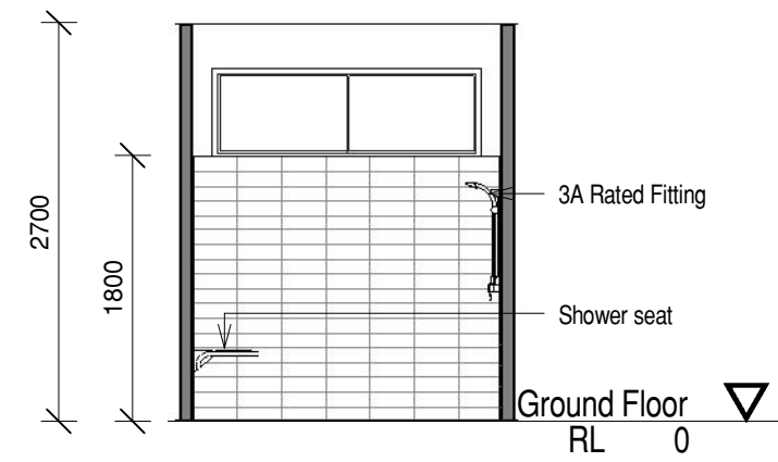
D Bathroom 2 - Elevation D 1 : 50
