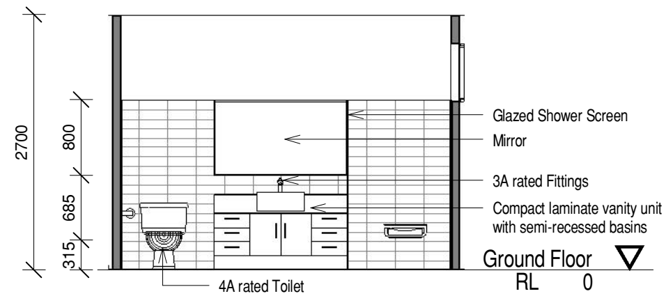
C Bathroom 2 - Elevation C 1 : 50
