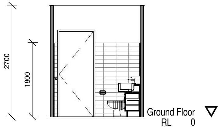
B Bathroom 2 - Elevation B 1 : 50
