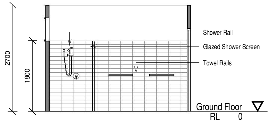
A Bathroom 2 - Elevation A 1 : 50
