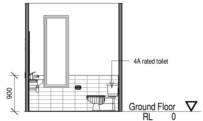
C PWD - Elevation C 1 : 50
