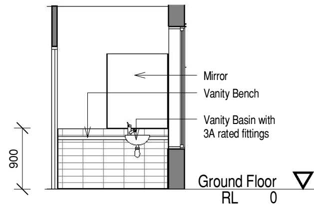
B PWD - Elevation B 1 : 50
