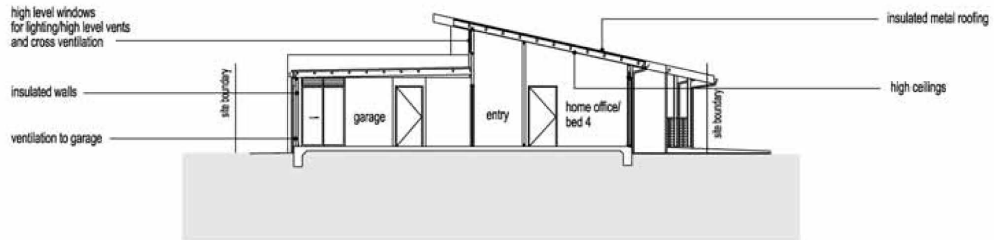
section b-b
